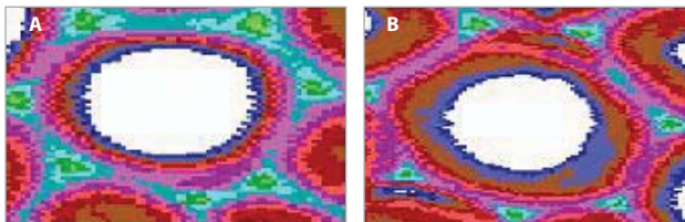
Figure 2. Topochemical distribution of lignin in rind fibers of sugarcane (A) and 1-h chlorite delignified sugarcane (B). In these pictures, blue and brown colors means low lignin contents, while red-pink and light green colors means high lignin contents
